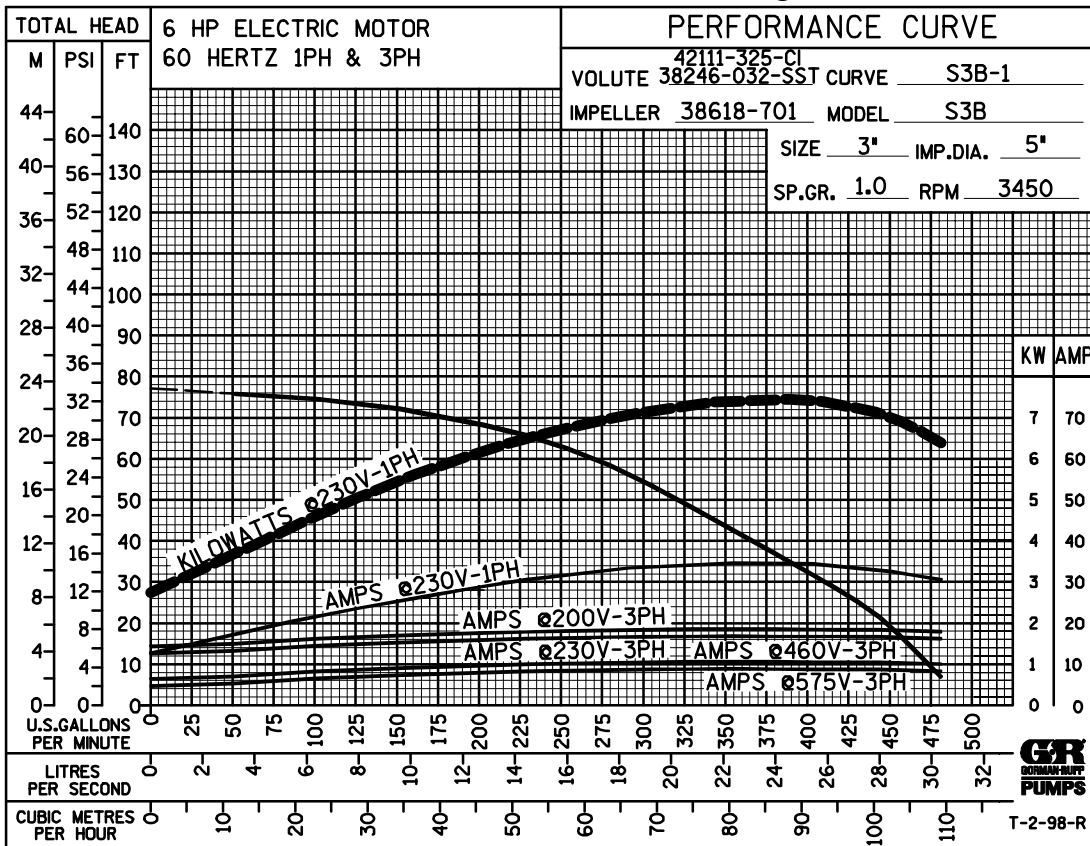
Performance Curve – Models S3B1 230V 1P And S3B1 230V/460V 3P
