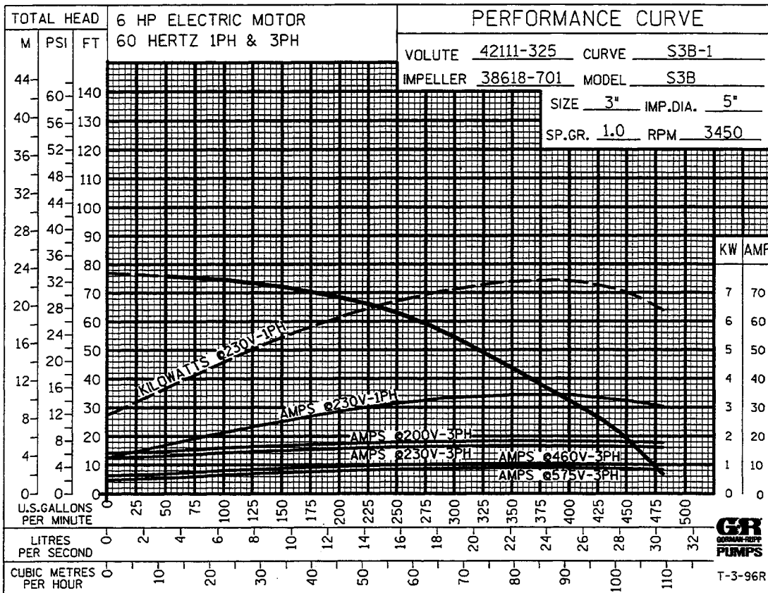
Performance Curve – Model S3B18 230V 1P
