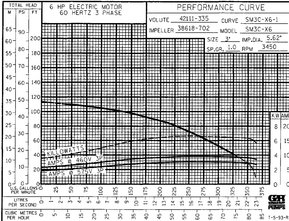
Performance Curve – Model SM3C1-X6 460/575/3
