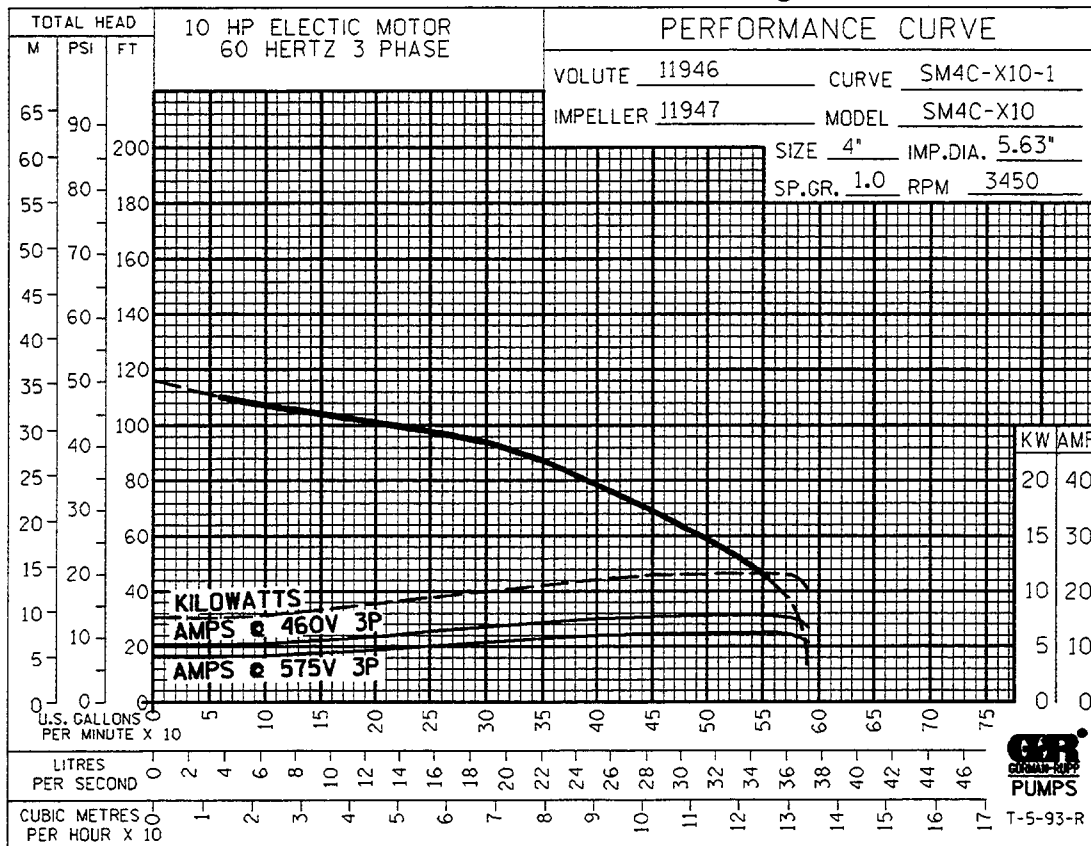
Performance Curve – Model SM4C18-X10 460/575/3
