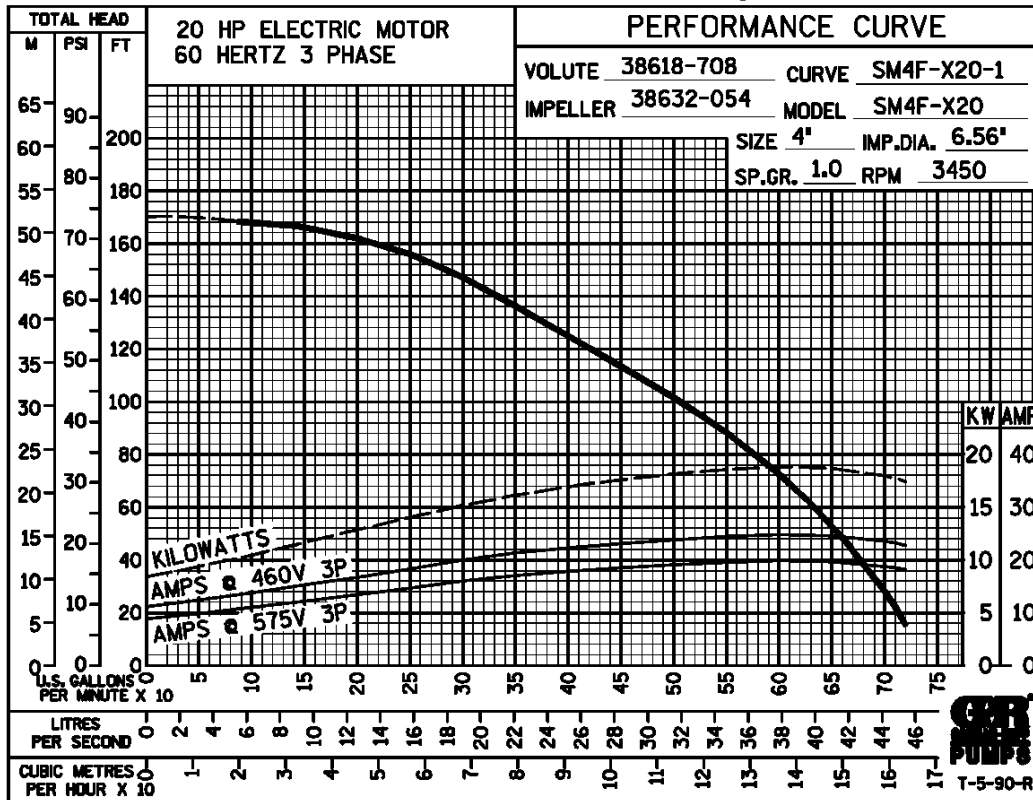
Performance Curve – Model SM4F1-X20 460/575/3
