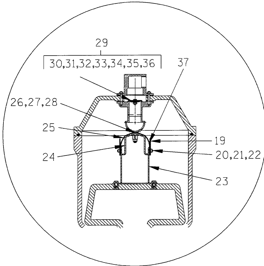
VALVE DETAIL
