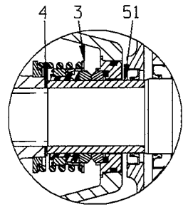
SEAL AREA DETAIL
