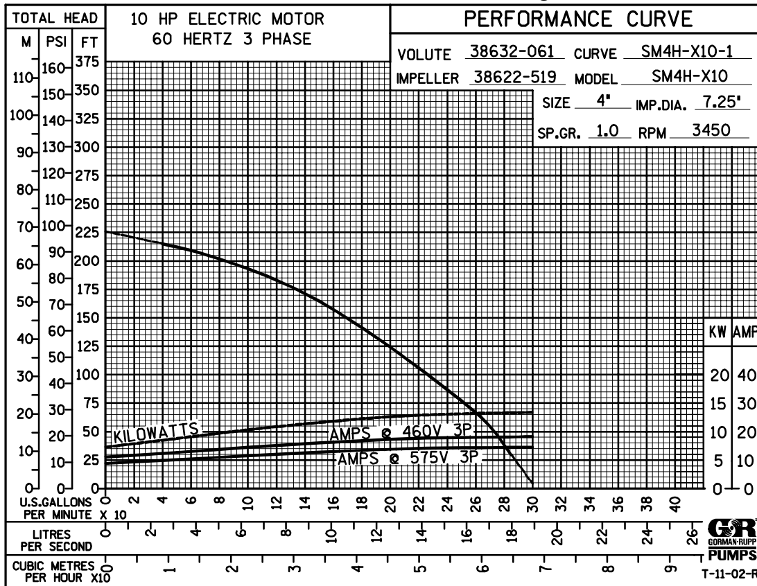
Performance Curve – Model SM4H18–X10 460/575/3
