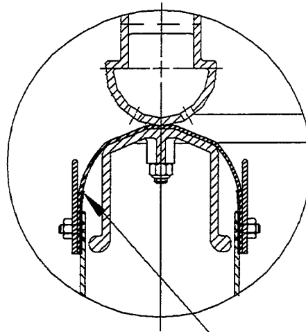
34 VALVE DETAIL
