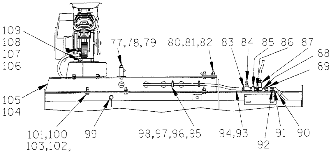
VENTURI SYSTEM AND MISC. HARDWARE
