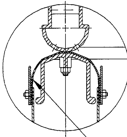
VALVE DETAIL
