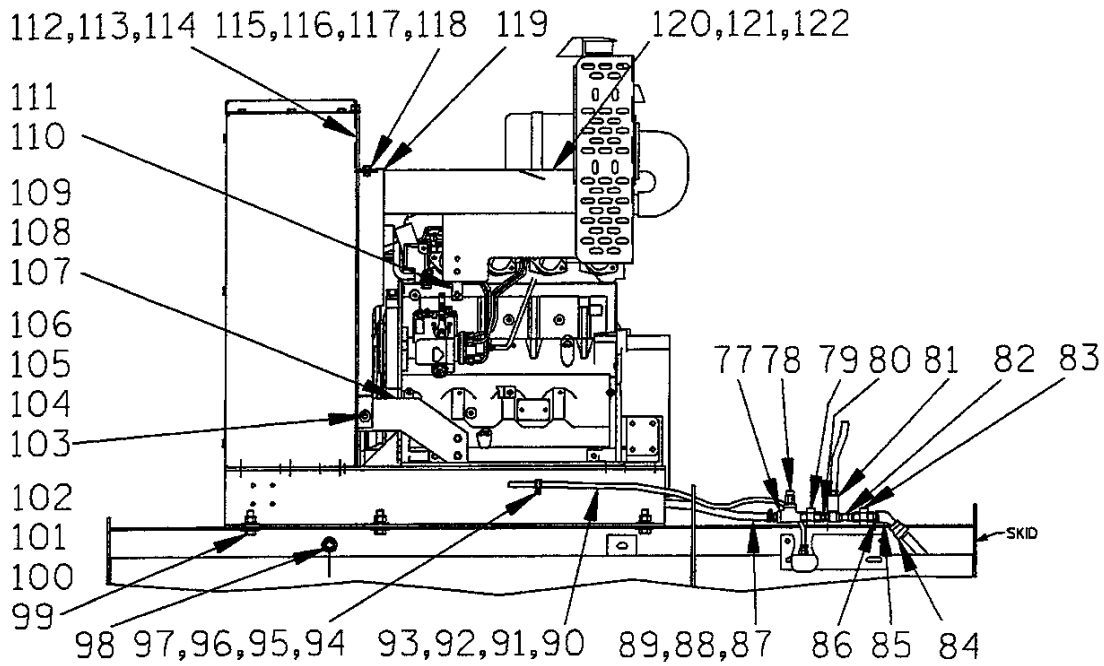
VENTURI SYSTEM AND BELT GUARDS
