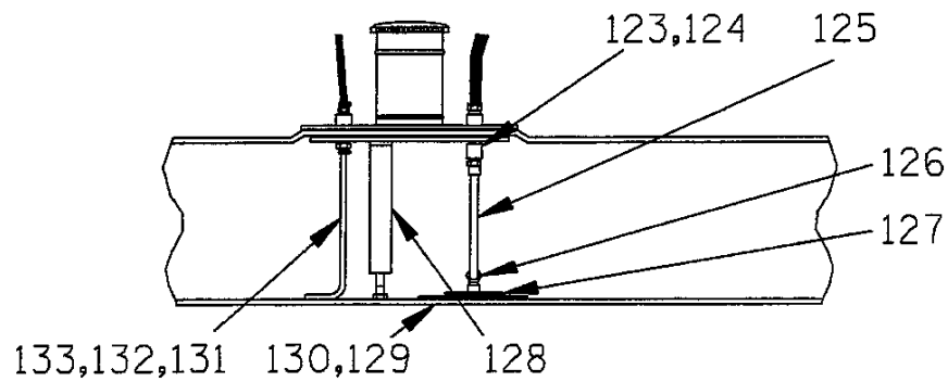
FUEL PICK-UP SYSTEM
