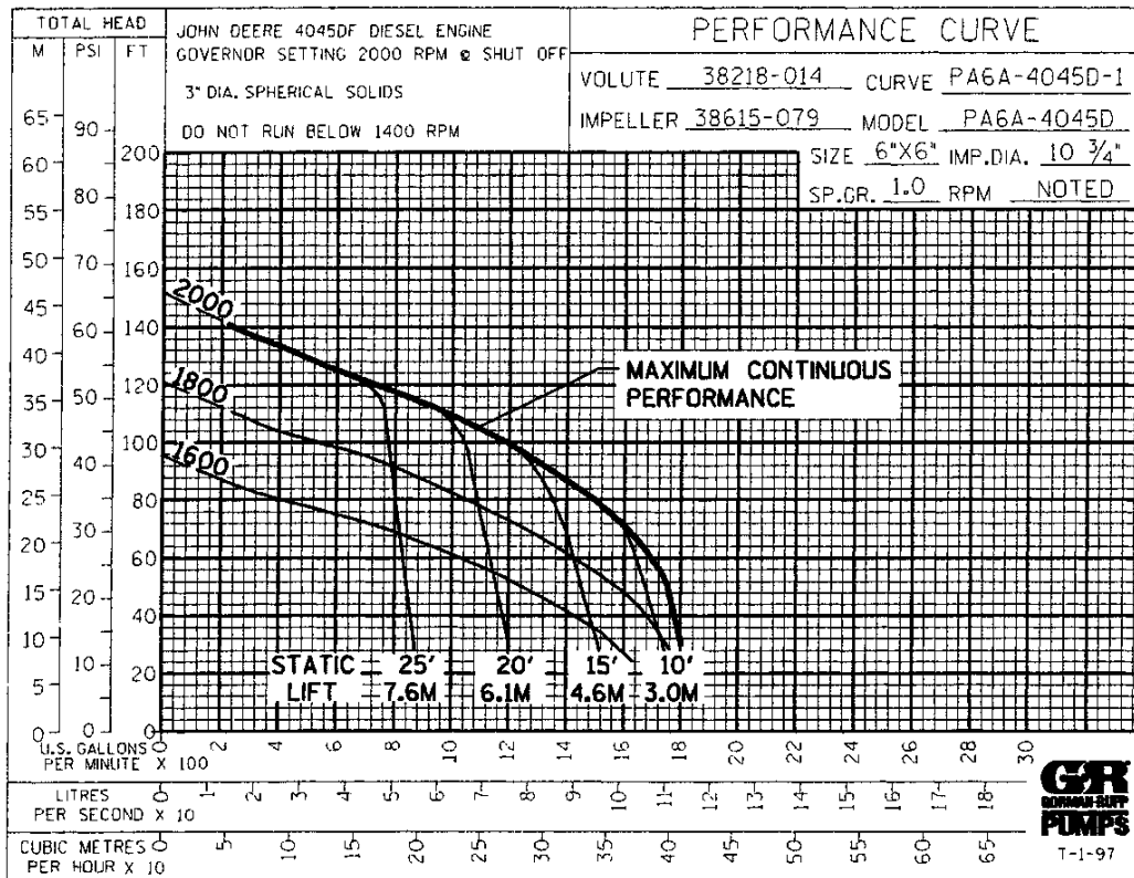
Performance Curve – Model PA6A60-4045D
