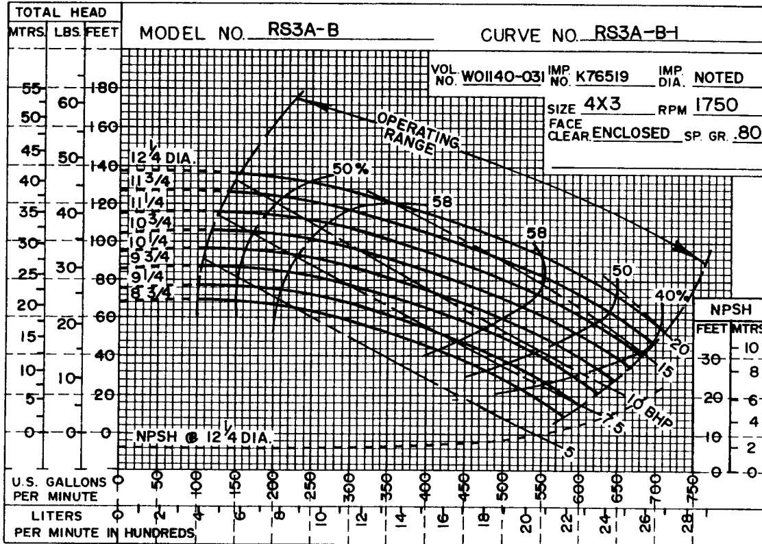
Performance Curve - Model RS3A31-B
