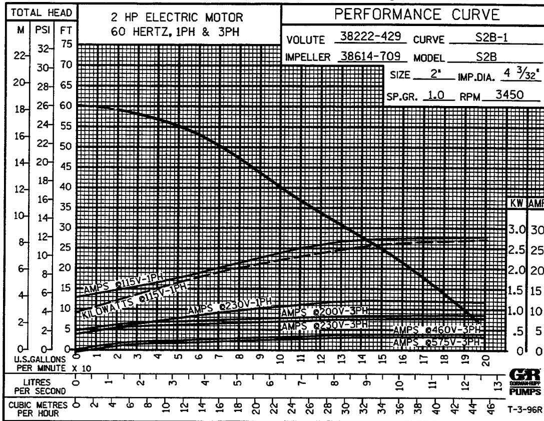
Performance Curve – Model S2B65-E2 115/1
